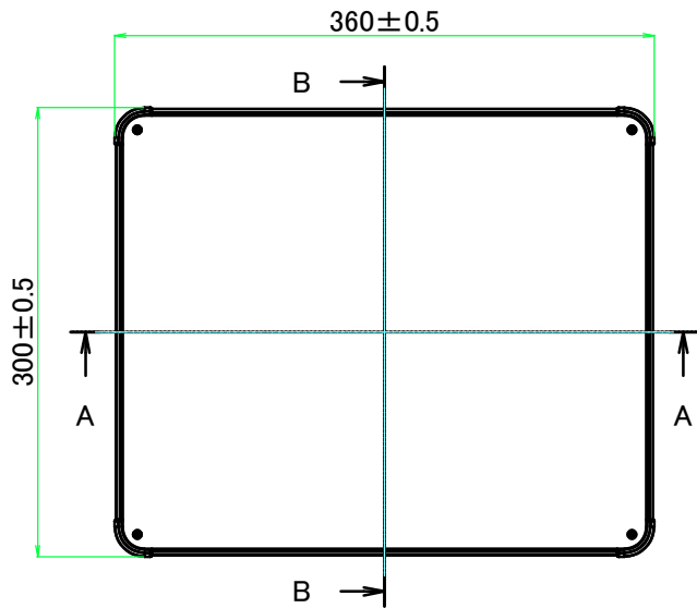
E view
